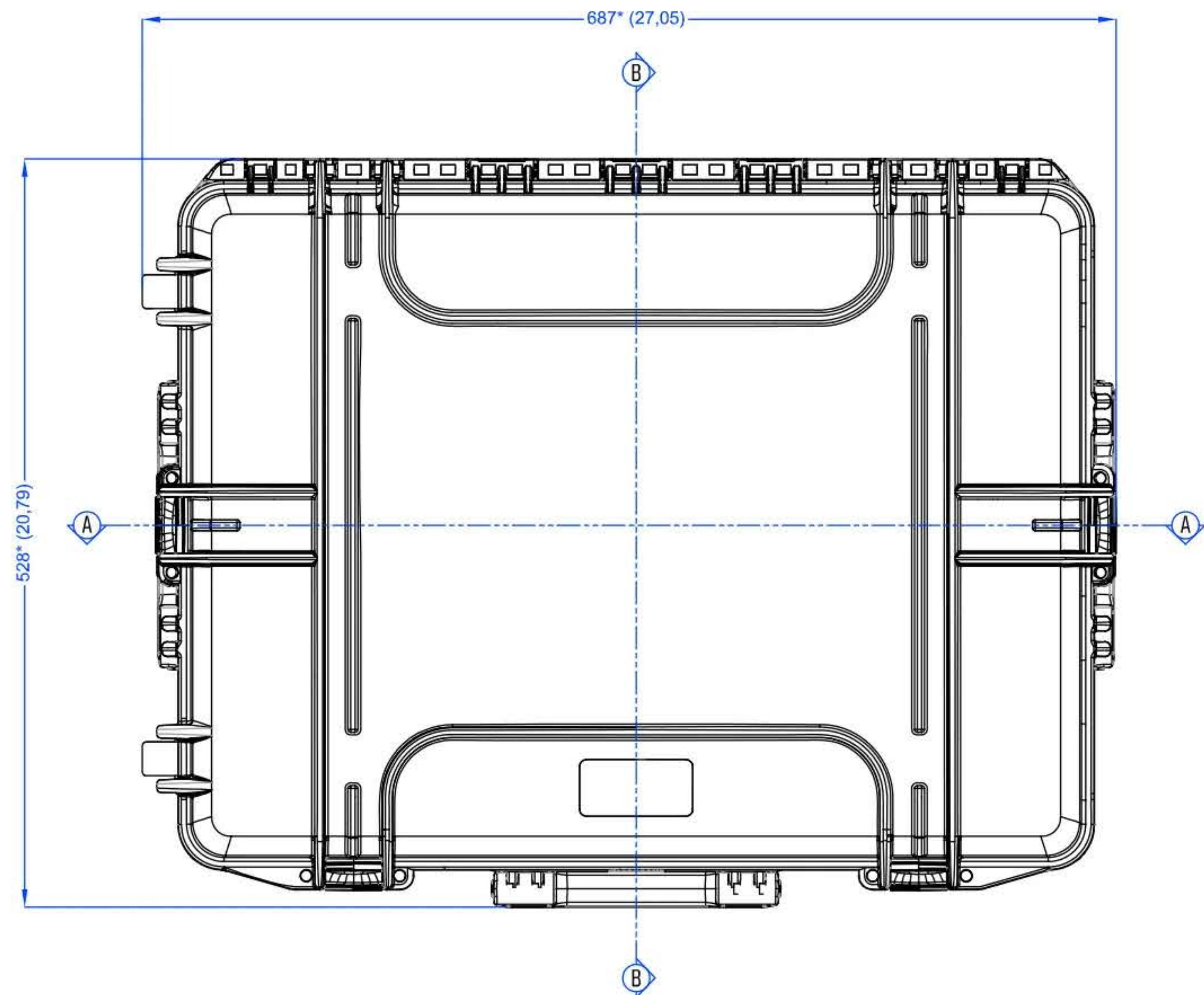
Vista Coperchio Lid View
